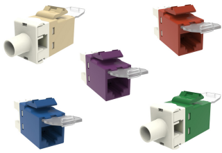
SL-Series Modular Jack, RJ45, Cat6 Unshielded, with Dust Cover
